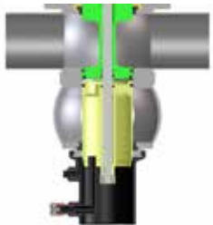
Valve Open
